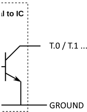
Transistor output
