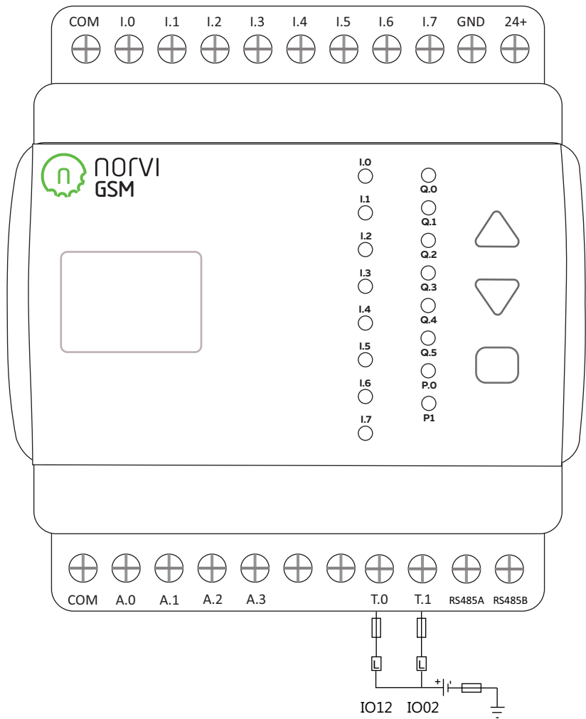
Transistor output
